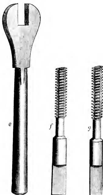
FIG. 132.—SPANNER AND TAPS FOR ROUGHING.
